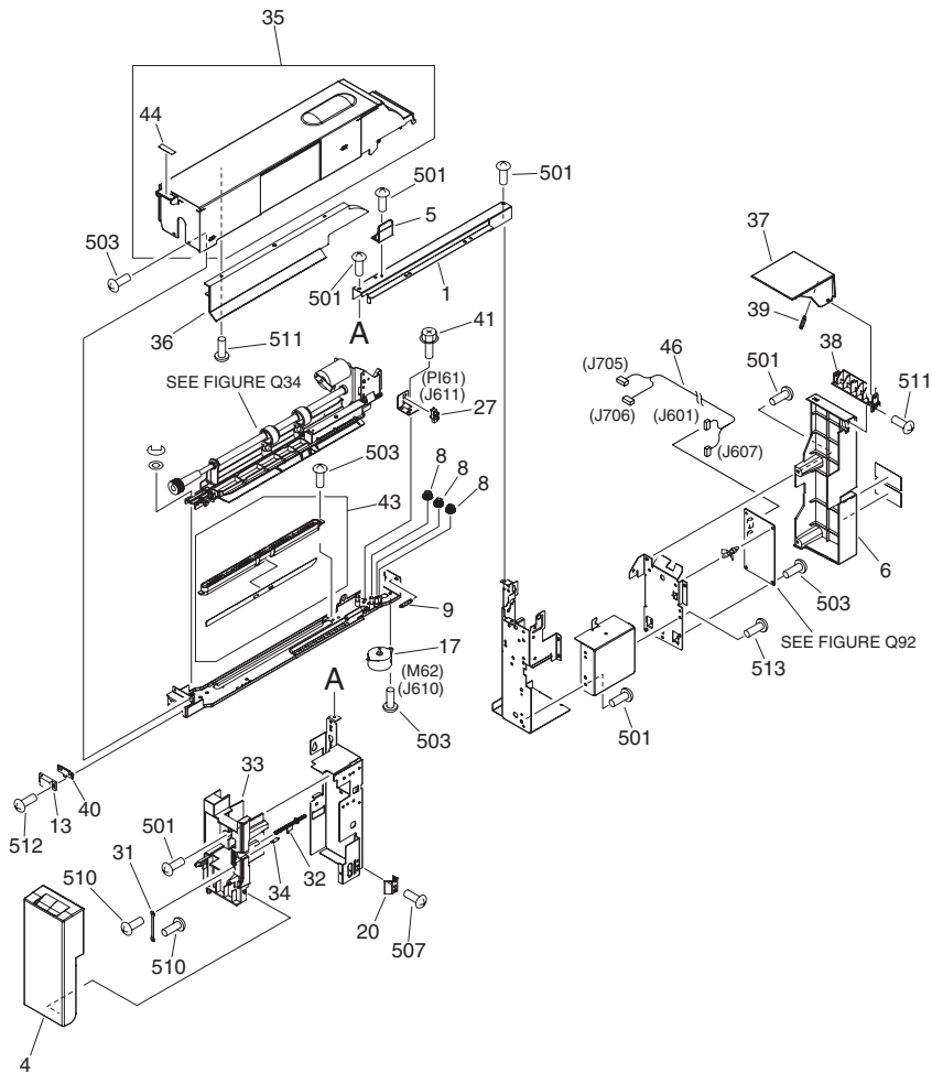
FIGURE Q12 PUNCH MAIN BODY
